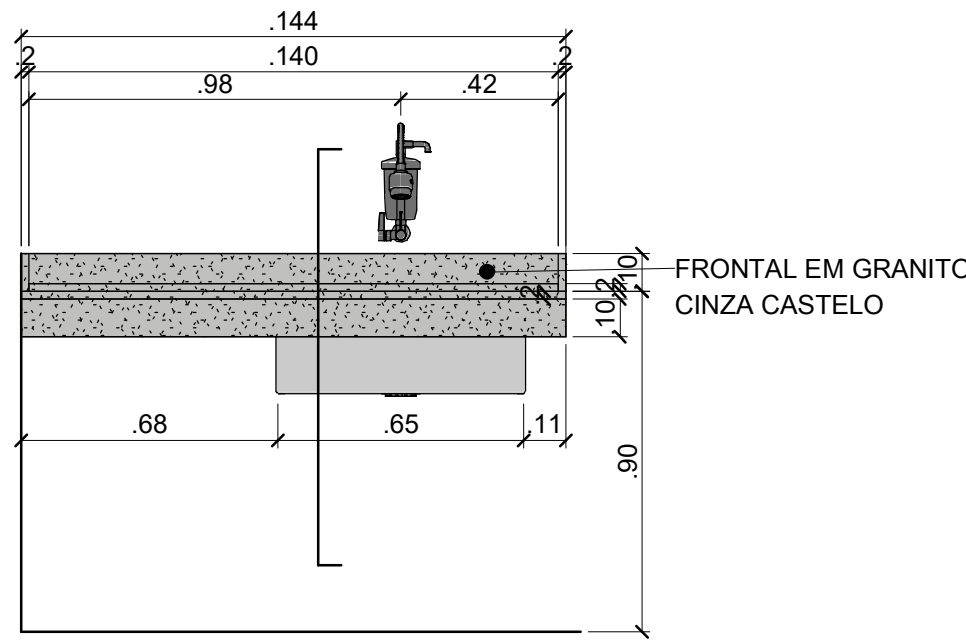
6 BG7: VISTA FRONTAL 1 : 20
