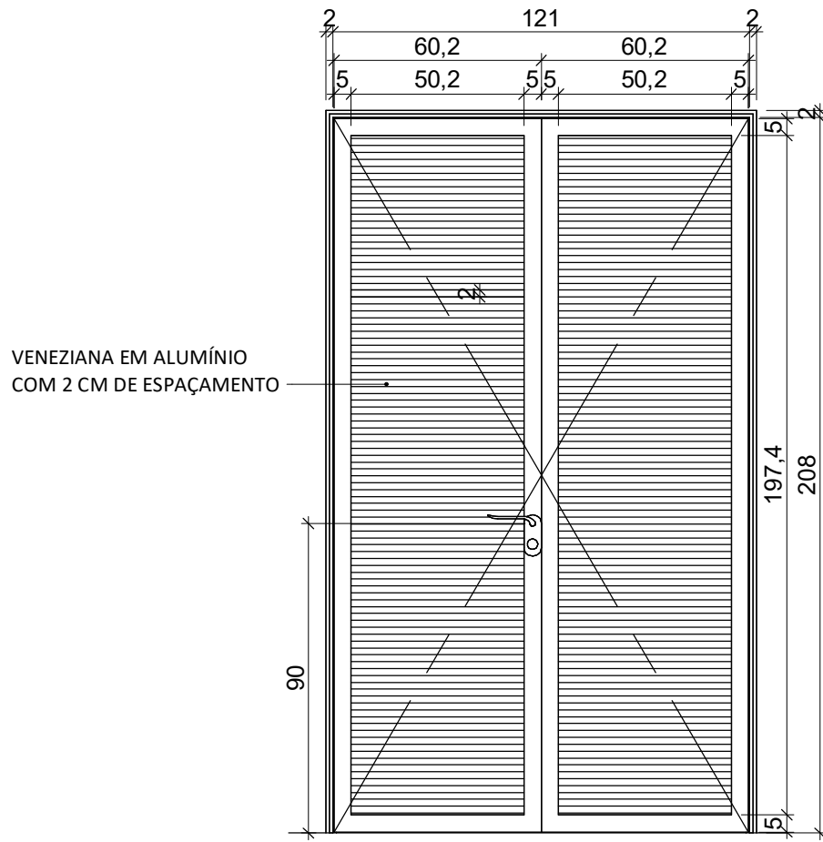
1 P05 - VISTA FRONTAL 1 : 20
