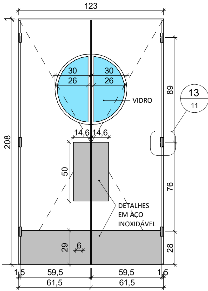
10 P04 - VISTA FRONTAL 1 : 20
