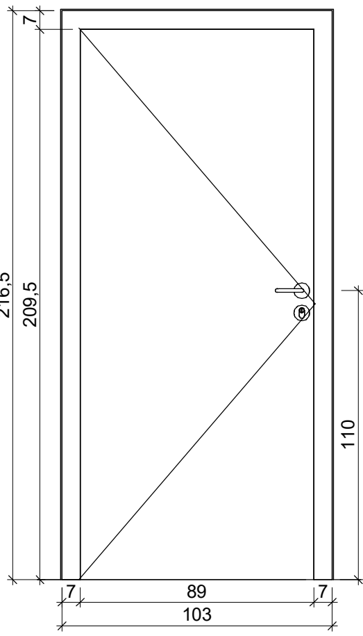
7 P03 - VISTA FRONTAL 1 : 20
