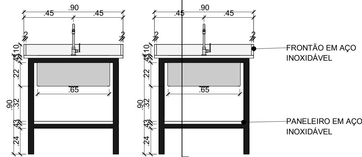
2 BG3: VISTA FRONTAL 1 : 20
